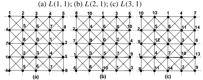
Figure 6 General patterns for L(h, k) -labellings of G_8 :
