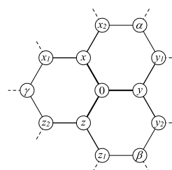
Figure 3 Neighbourhood of a node labelled 0 in G_3
