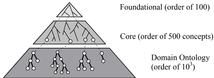
Figure 1. The three levels of generality of a Domain Ontology.
