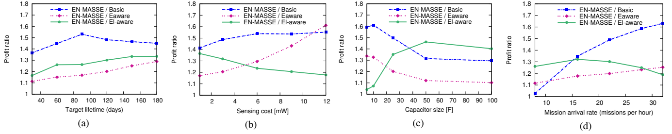
Fig. 2. Simulation results: performance improvement for varying (a) target lifetime, (b) sensing cost, (c) capacitor size and (d) mission arrival rate.
