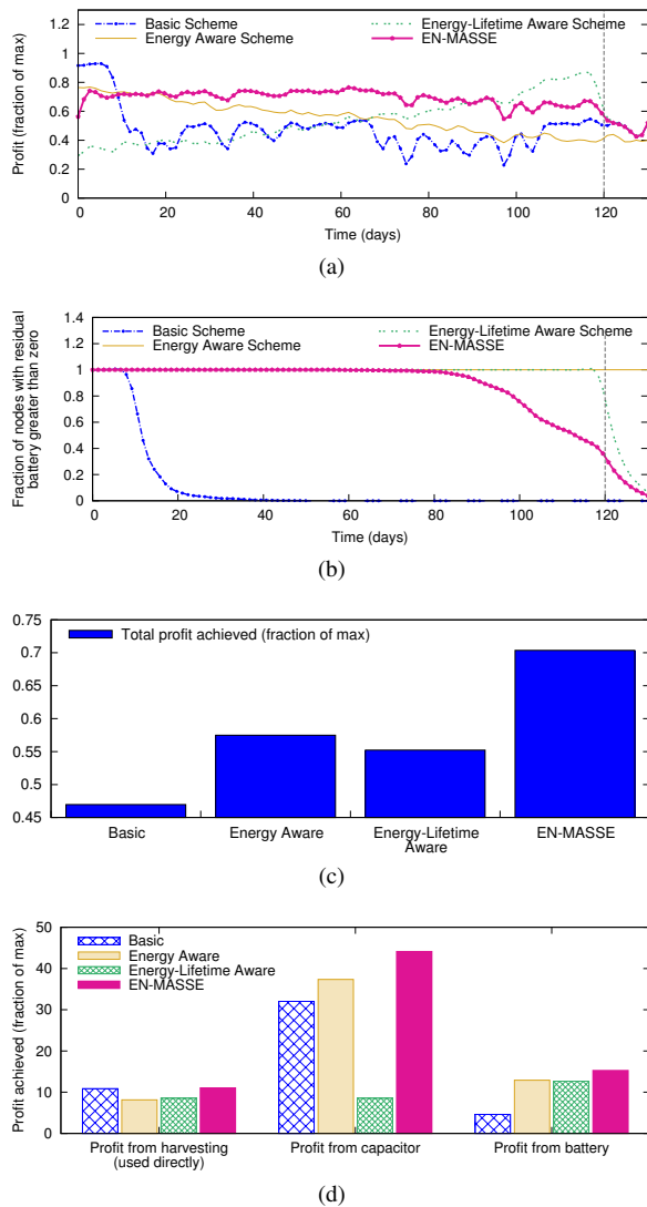
Fig. 1. Simulation results for a sample scenario: (a) fraction of achieved profits per time slot, (b) fraction of nodes with a residual battery greater than zero, (c) total profit achieved at target lifetime (as a fraction of maximum) and (d) total profit achieved per energy source (as a fraction of maximum).
